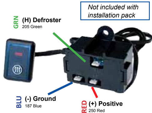
Connectors on ThermaSync control
