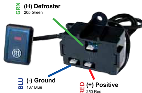
ThermaSync Defroster Control
